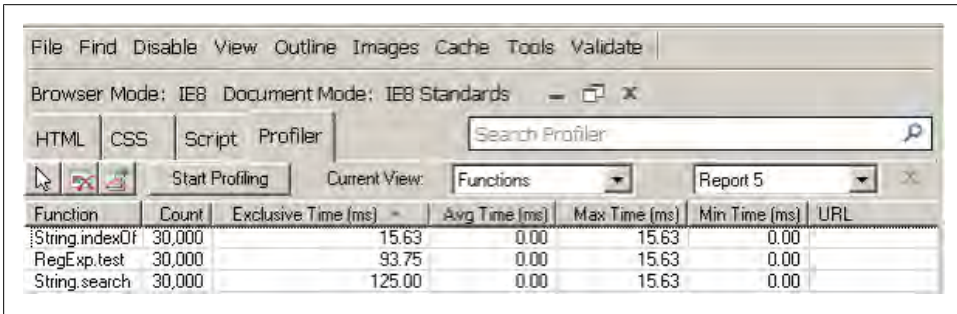
Figure 10-5. Profile results for native methods
